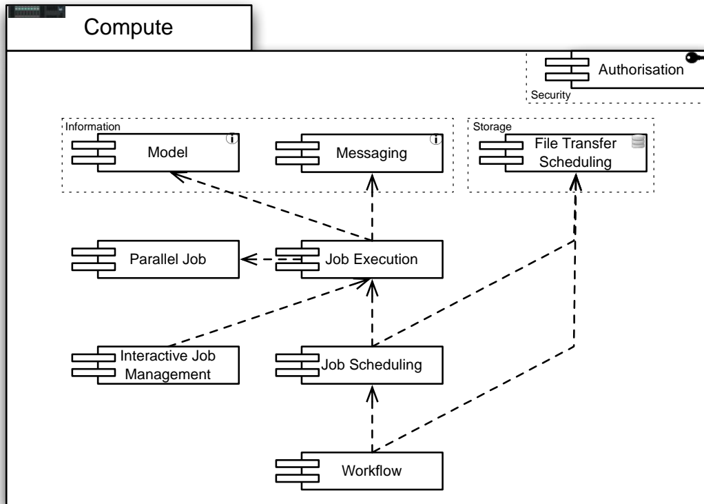
Figure 5: Dependencies for Compute Capabilities
