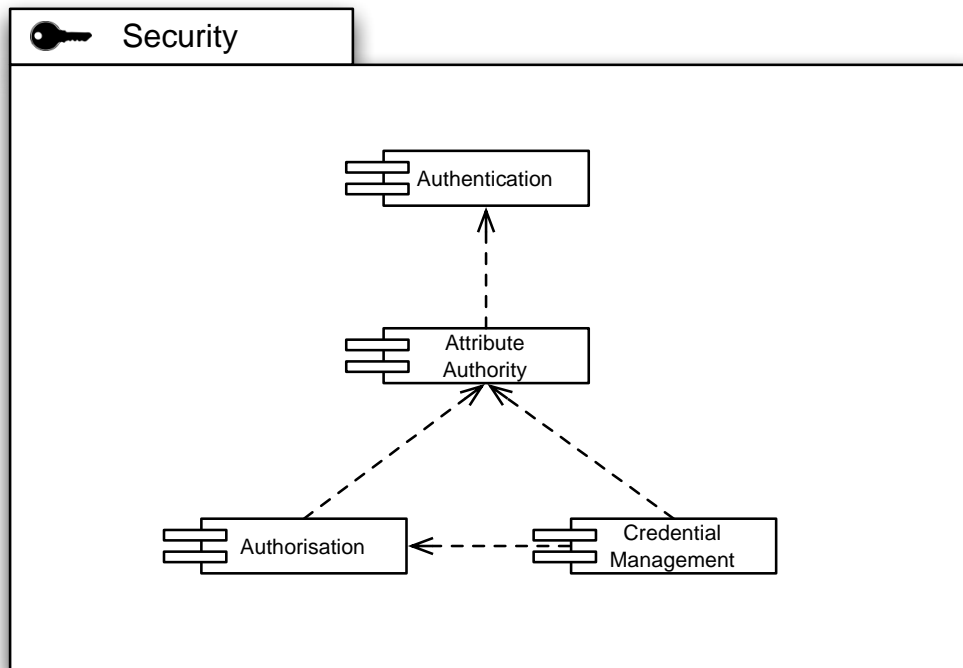
Figure 1: Dependencies of Security Capabilities.
