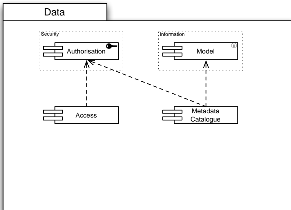
Figure 4: Dependencies of Data Capabilities
