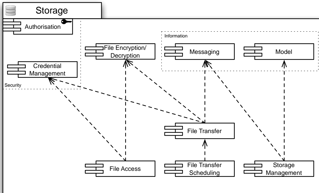
Figure 3: Dependencies of Storage Capabilities
