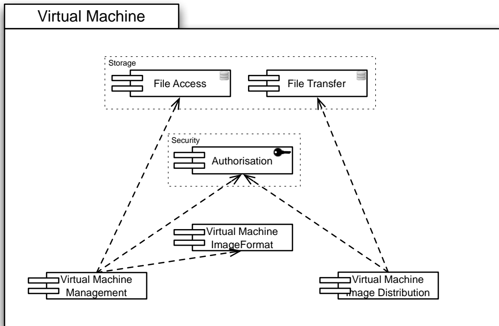
Figure 7: Dependencies of Virtualisation Capabilities
