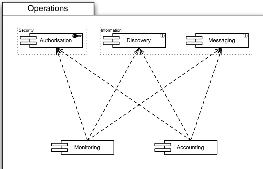
Figure 6: Dependencies of the Operations Capabilities
