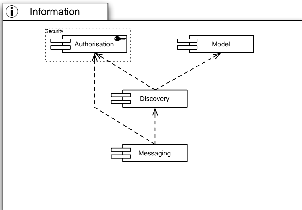
Figure 2: Dependencies of Information Capabilities
